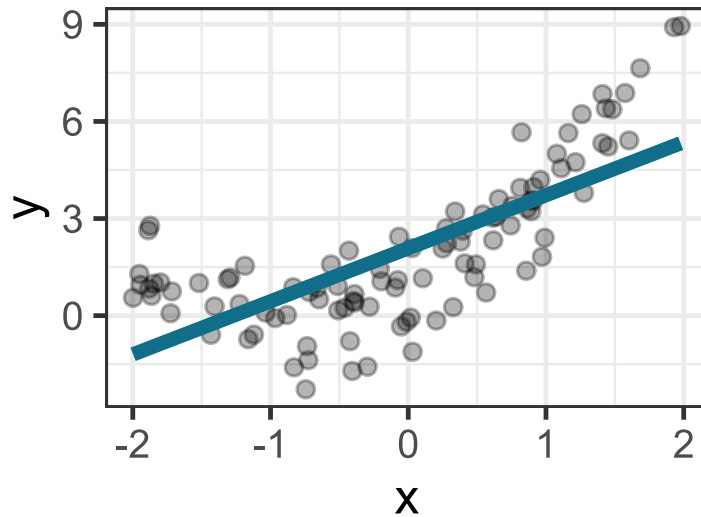
Underfitting
