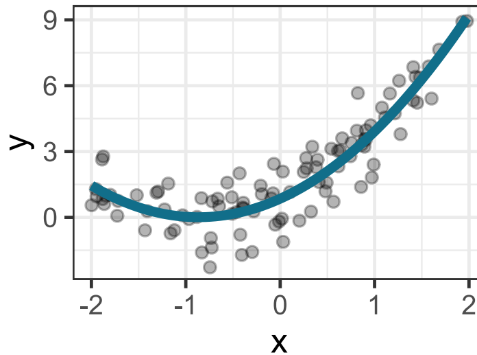
Just right?
