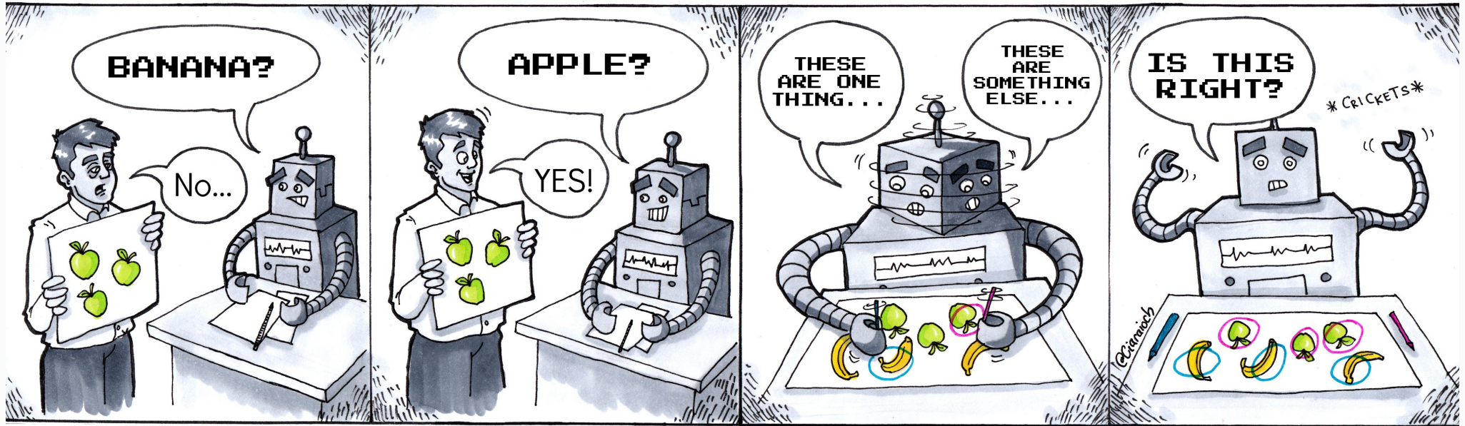
Supervised Learning
