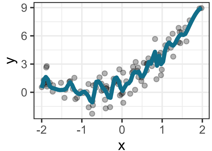
Overfitting
